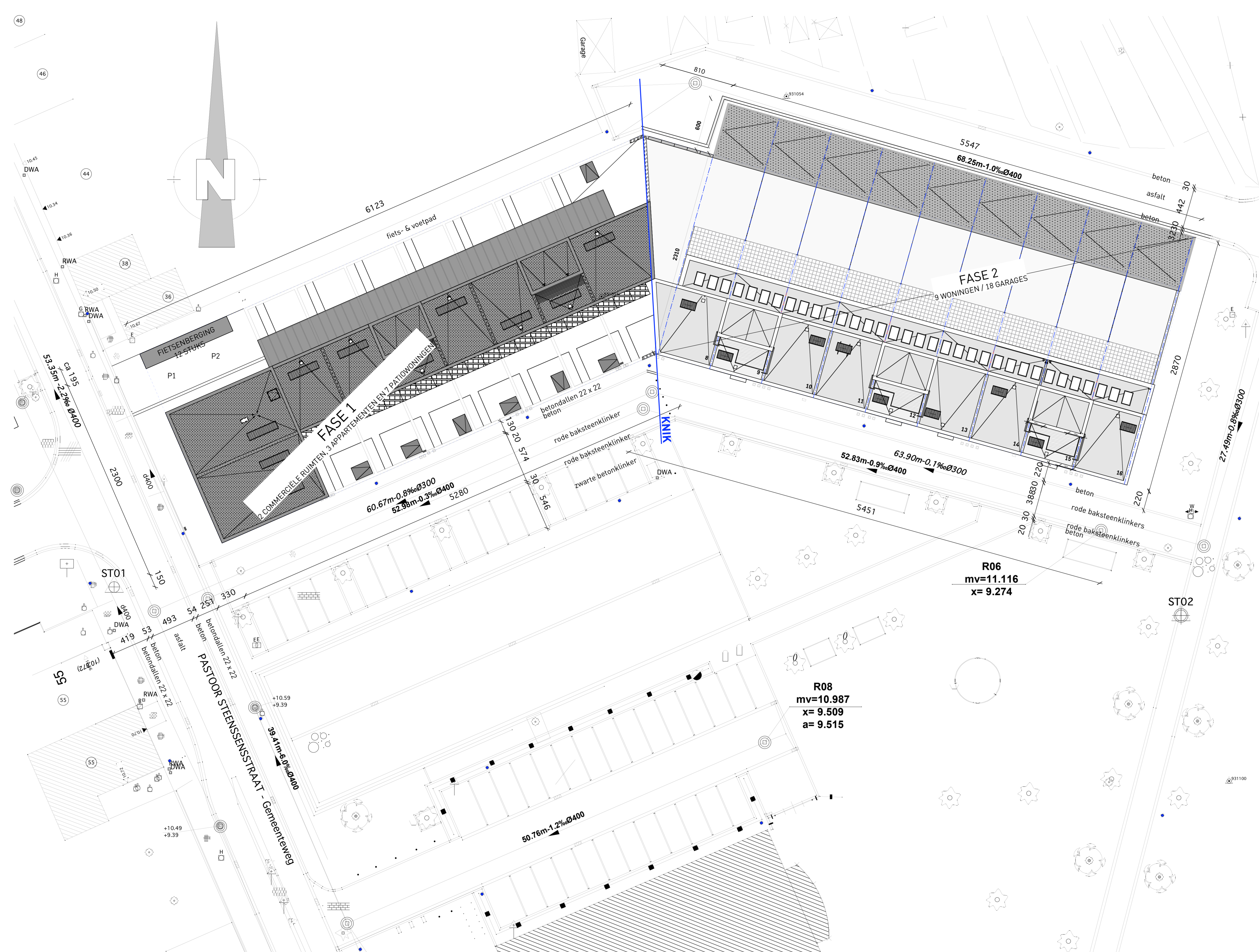
INPLANTINGSPLAN 1:200
